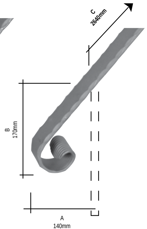
Martellato / Hammered Art.12.P1.017 \neq 40 x 8 mm Art.12.P1.018 \neq 50 x 10 mm
