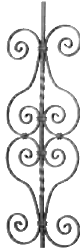
H.950 X L.275 mm. Art. 05.088 □12 ≡12 X 6
