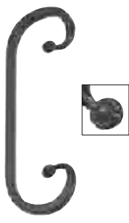
Liscio / Smooth H.190 X L.65 mm. Art. 01.401 □ 8 X 8
